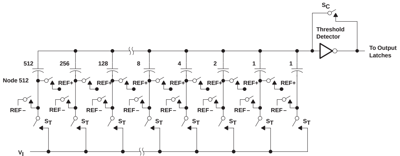
Figure 1. Simplified Model of the Successive-Approximation System
