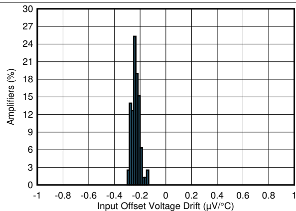
Figure 2. Offset Voltage Drift (-40°C to 125°C)
