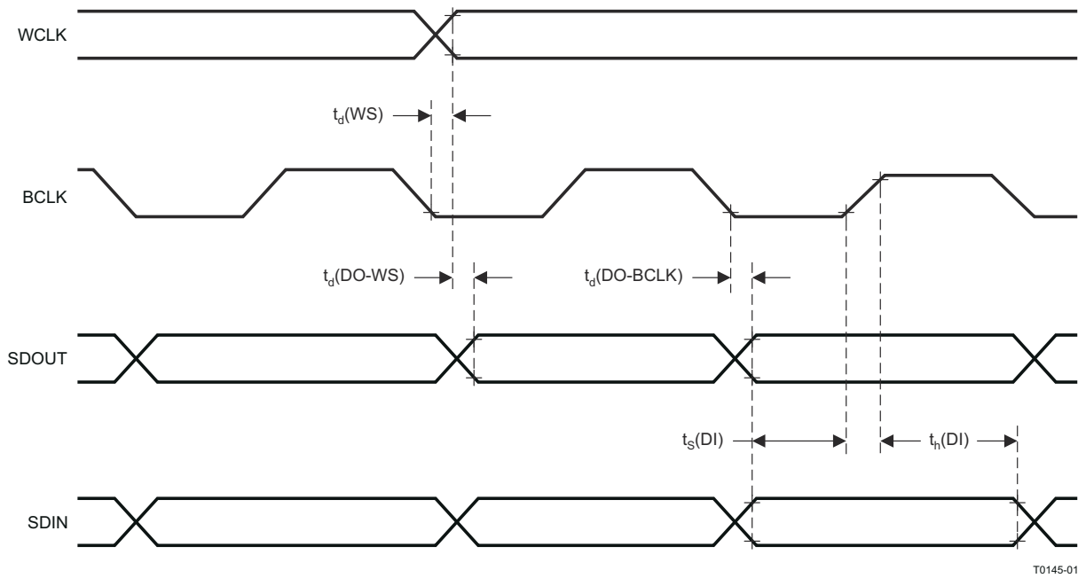
Figure 8-1. I²S, LJF, RJF Timing in Master Mode
