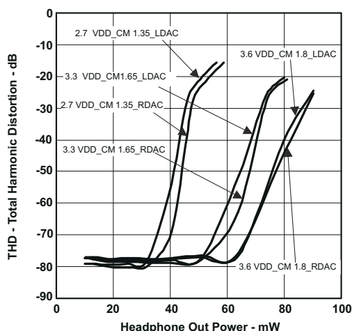
Figure 11-2. Total Harmonic Distortion vs Headphone Out Power
