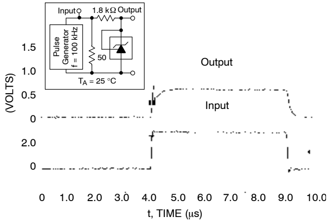
Figure 17. Pulse Response
