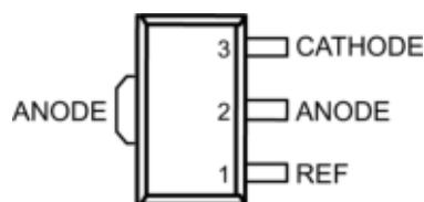
Figure 4-4. PK (SOT-89) Package (Top View)
