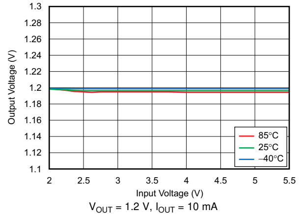
Figure 4. Line Regulation
