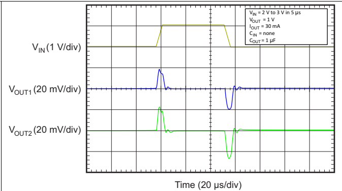
Figure 14. Line Transient
