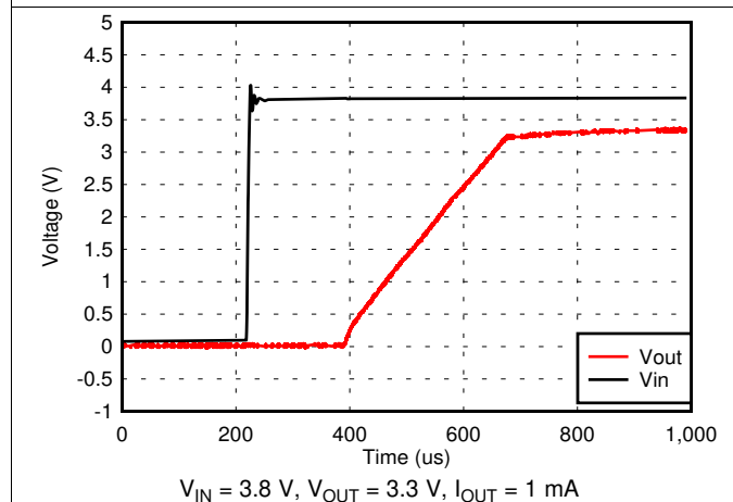
Figure 23. V_{IN} Power-Up
