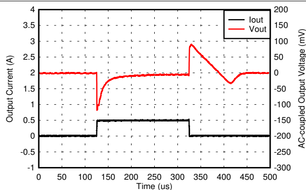
Figure 5-20. 3.3-V, 1-mA to 500-mA Load Transient
