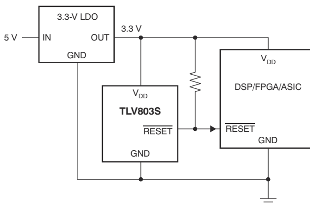
Typical Application
