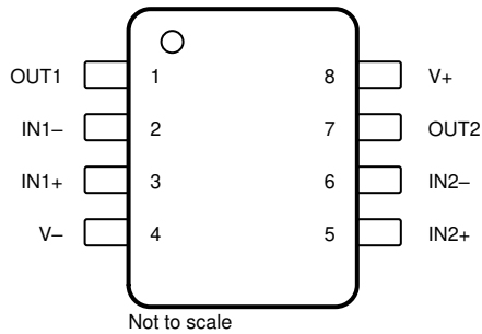
Figure 5-6. TLV9062 D, DGK, PW, or DDF Package, 8-Pin SOIC, VSSOP, TSSOP, or SOT-23 (Top View)
