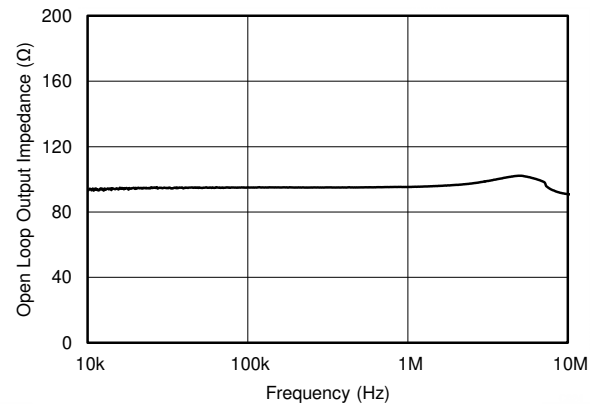
Figure 6-22. Open-Loop Output Impedance vs Frequency
