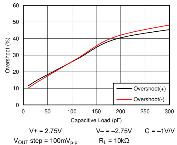
Figure 6-24. Small-Signal Overshoot vs Load Capacitance
