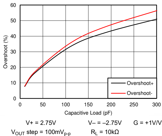
Figure 6-23. Small-Signal Overshoot vs Load Capacitance
