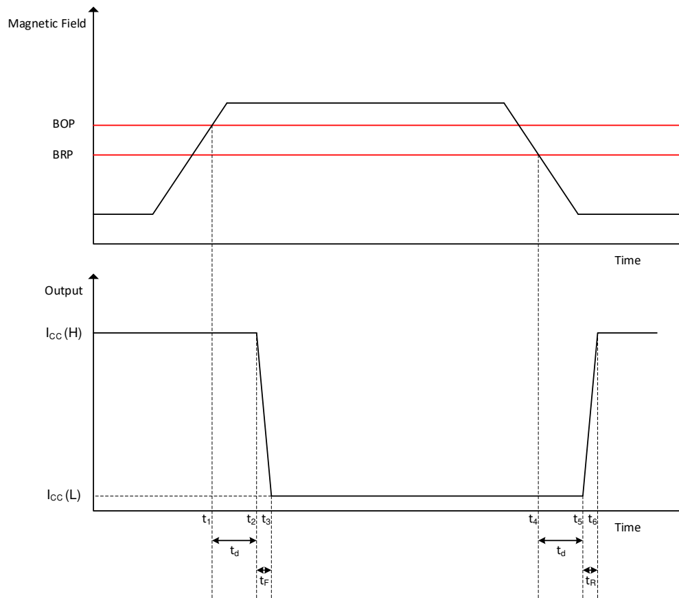
Figure 8-8. Propagation Delay
