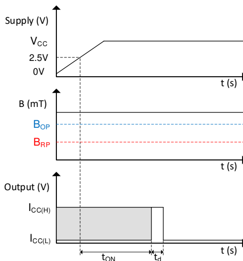
Figure 8-5. Power-On Time When B > B_{OP}
