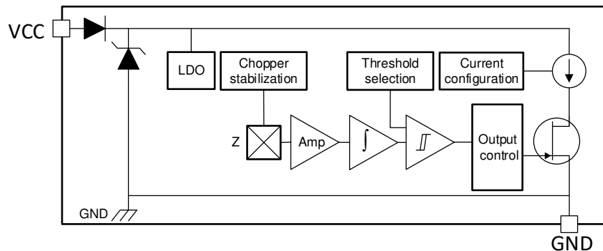
Figure 8-1. Block Diagram
