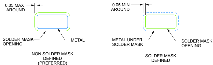
SOLDEMASK DETAILS
