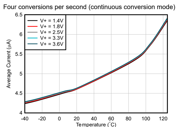
Figure 6-12. Average Quiescent Current vs Temperature
