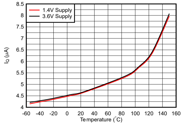
Figure 6-5. Average Quiescent Current vs Temperature
