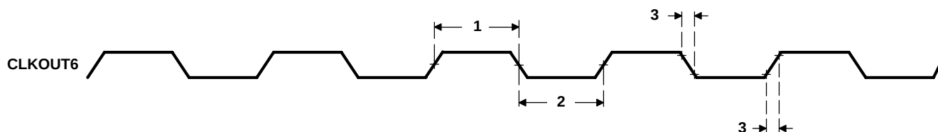
Figure 4–15. CLKOUT6 Timing
