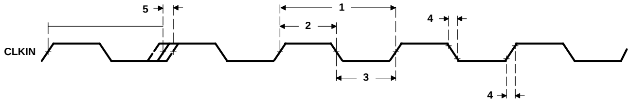
Figure 4-13. CLKIN Timing
