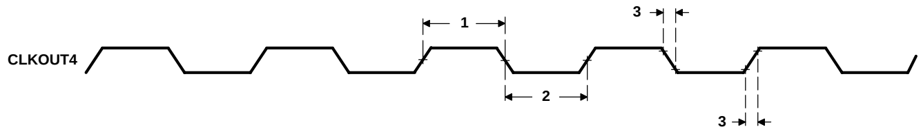
Figure 4-14. CLKOUT4 Timing
