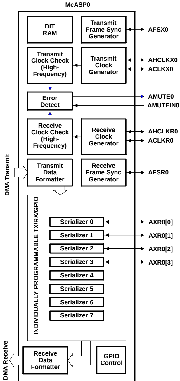
Figure 4-34. McASP0 Configuration
