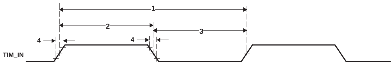
Figure 6-74. Timer Timing
