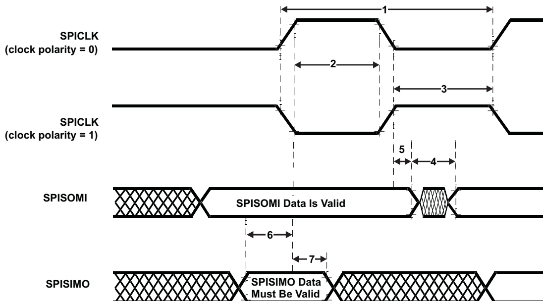
Figure 7-21. SPI Slave Mode External Timing (CLOCK PHASE = 1)
