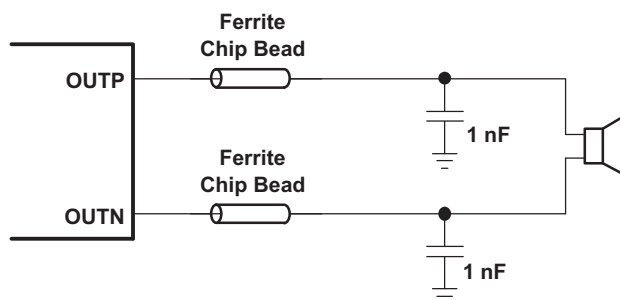
Figure 40. Typical Ferrite Chip Bead Filter (Chip Bead Example)
