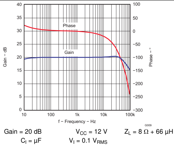
Figure 9. Gain/Phase vs Frequency
