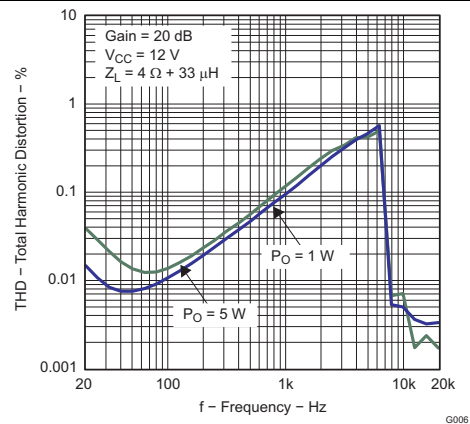
Figure 4. Total Harmonic Distortion vs Frequency (BTL)
