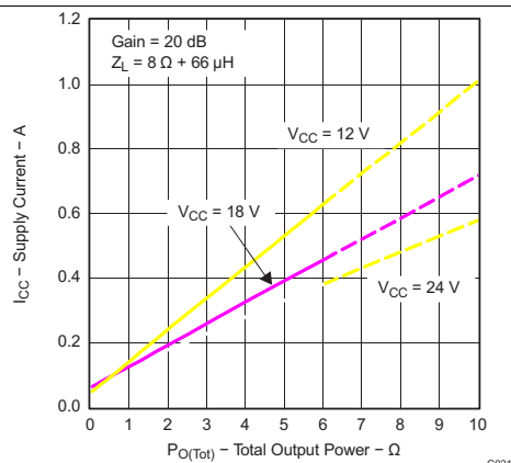
Figure 20. Supply Current vs Total Output Power (BTL)
