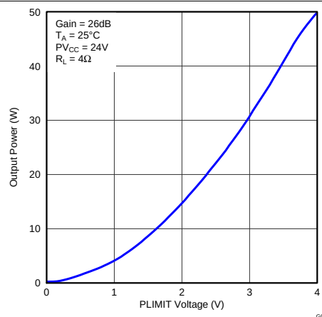
Figure 11. Output Power (BTL) vs Plimit Voltage
