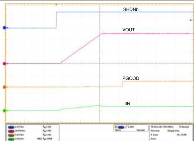
Figure 9-7. Turn ON Using \overline{\text{SHDN}} Control
