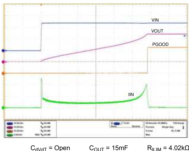
Figure 8-2. Thermal Regulation Loop Response During Power Up With Large Capacitive Load
