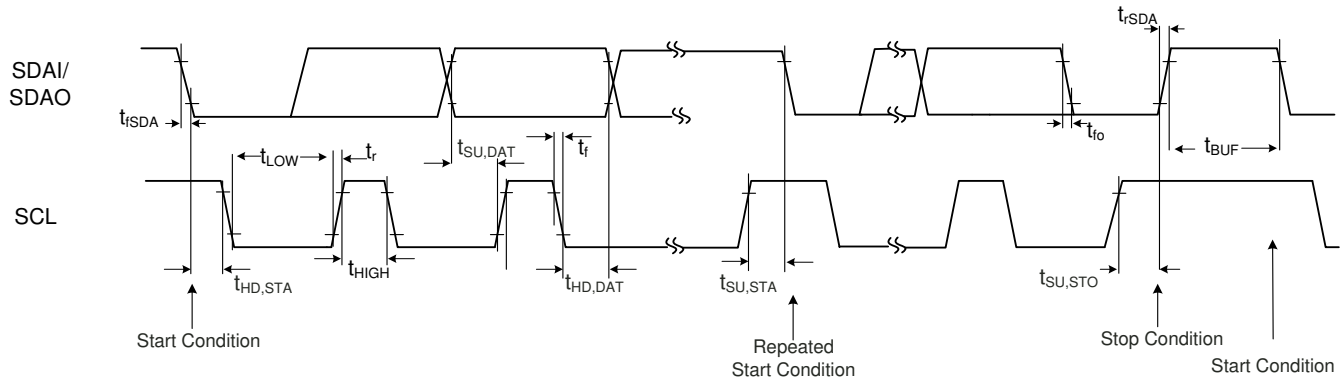
Figure 8-1. I²C Timings
