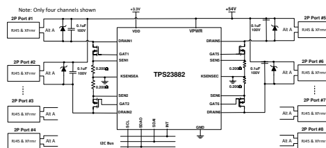
Simplified Schematic
