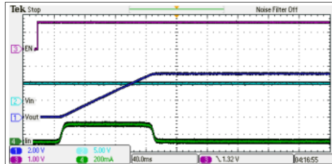
Figure 43. Output Ramp Up
