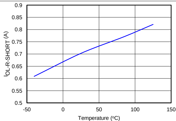
Figure 21. I_{OL} , I_{SC} vs Temperature
