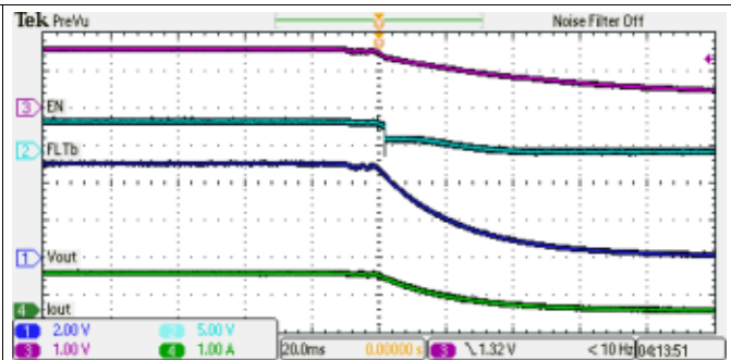
Figure 44. Hold-Up Power when VIN fails
