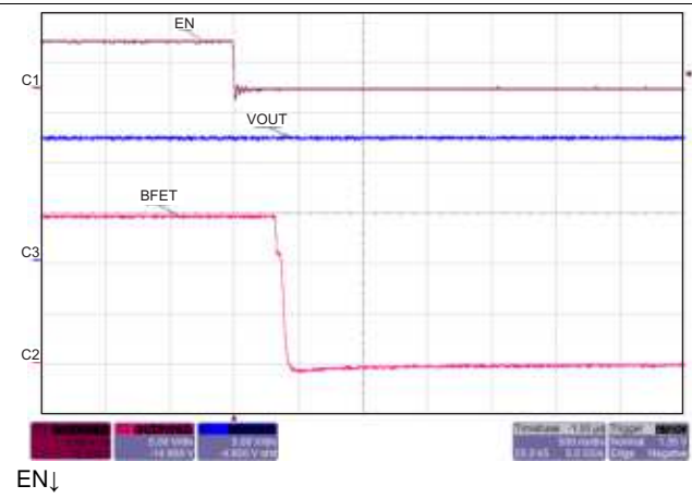
Figure 14. Turn Off Delay to BFET
