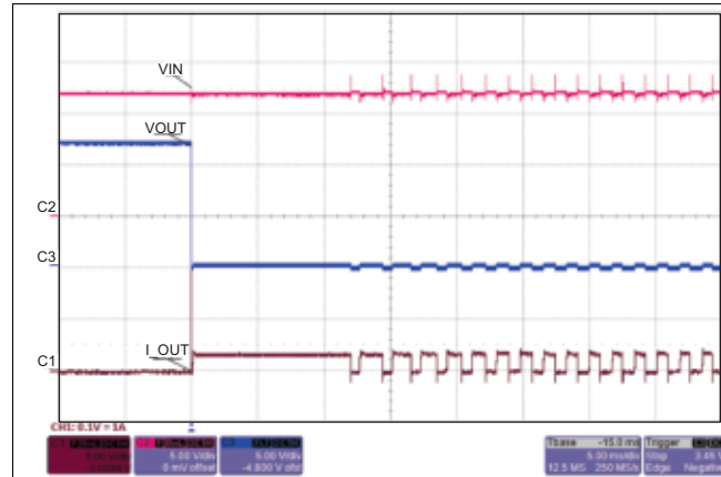
TPS2592BA
