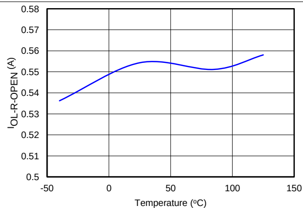
Figure 22. I_{OL} , I_{SC} vs Temperature
