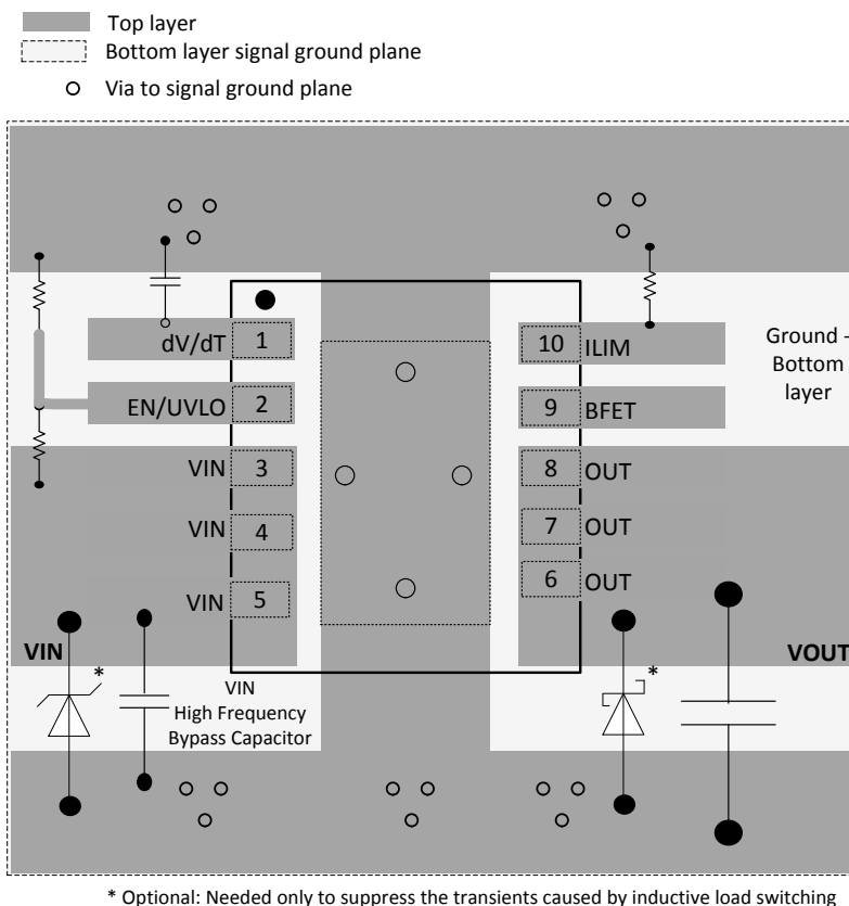
Figure 46. Layout Example
