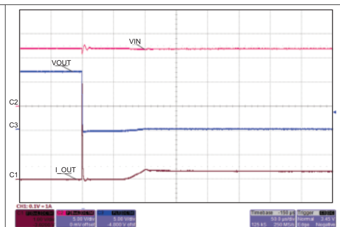
Figure 37. Fast-Trip and Current Limit Amplifier Response for Short Circuit
