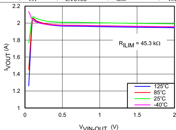
Figure 19. I_{OUT} vs V_{VIN-OUT}
