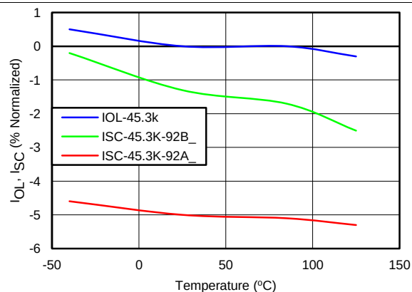
Figure 20. I_{OL} , I_{SC} vs Temperature
