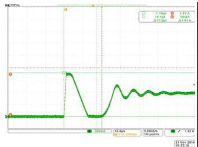
Figure 37. Hard Short-to-GND Waveform
