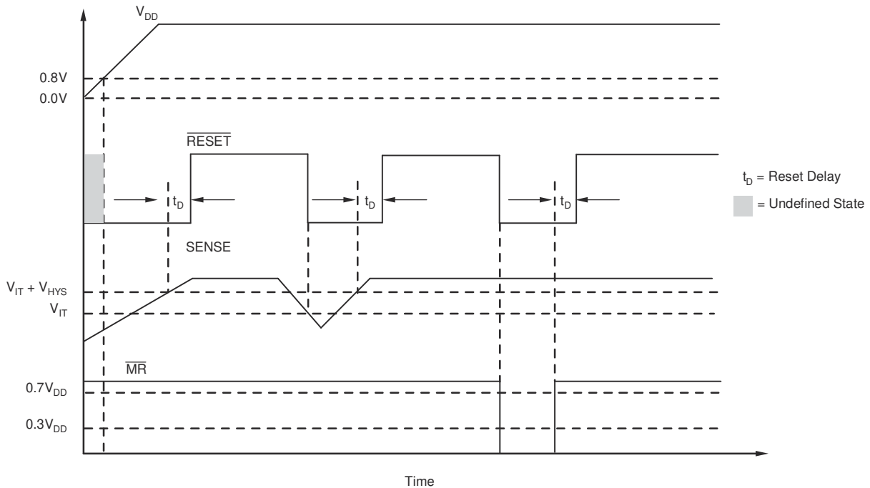
Figure 6-1. TPS3808 Timing Diagram Showing \overline{MR} and SENSE Reset Timing
