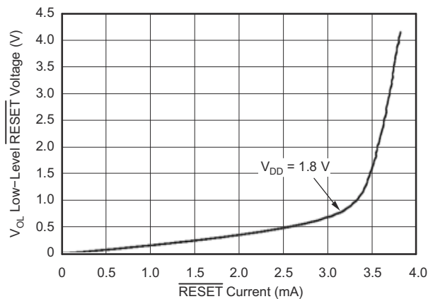
Figure 6-7. Low-Level RESET Voltage vs RESET Current
