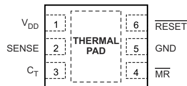
Figure 5-2. DRV Package 6-Pin (2.00mm × 2.00mm) WSON With Thermal Pad Top View
