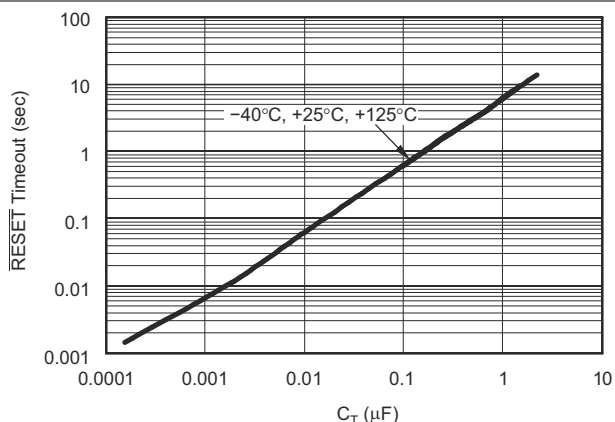
Figure 6-3. RESET Time-Out Period vs C_T
