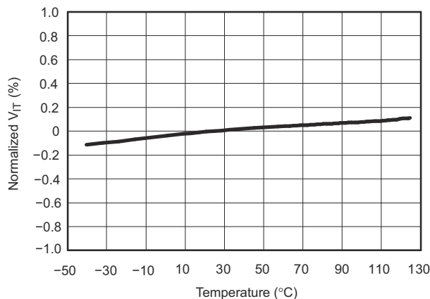
Figure 6-6. Normalized Sense Threshold Voltage ( V_{IT} ) vs Temperature
