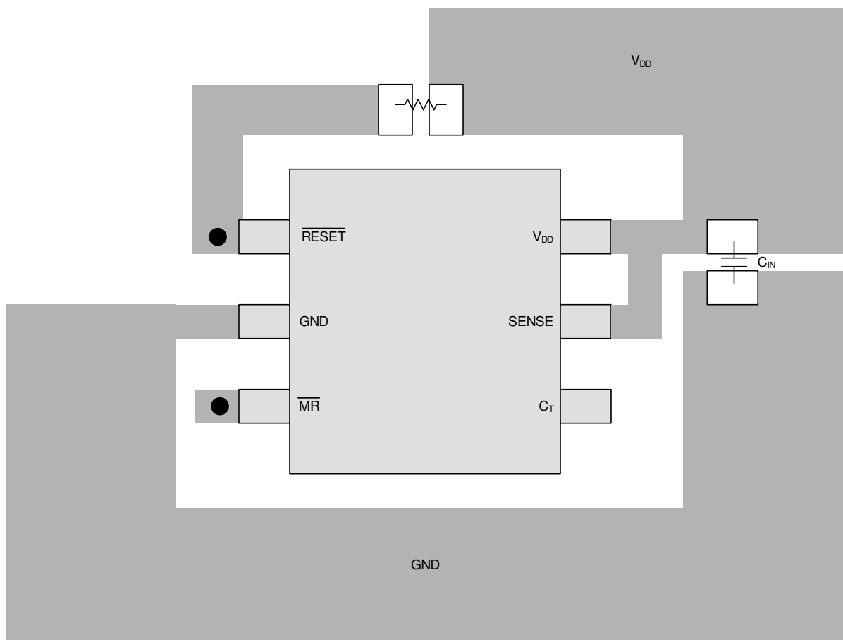
Figure 8-3. Layout Example for a 20ms Delay
