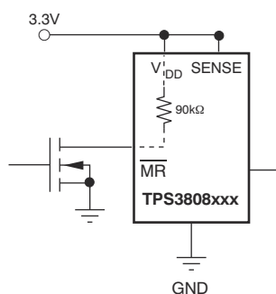
Figure 7-4. Using an External MOSFET to Minimize \text{I}_{\text{DD}} When \overline{\text{MR}} Signal Does Not Go to \text{V}_{\text{DD}}
