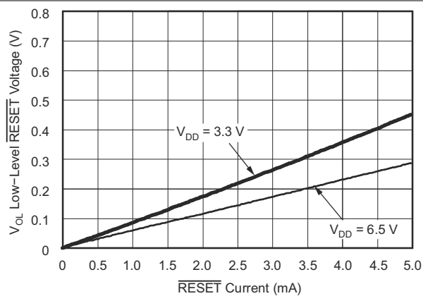
Figure 6-8. Low-Level RESET Voltage vs RESET Current
