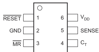
Figure 5-1. DBV Package 6-Pin SOT-23 Top View
