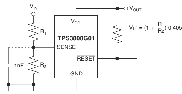
Figure 7-1. Using the TPS3808G01 to Monitor a User-Defined Threshold Voltage
