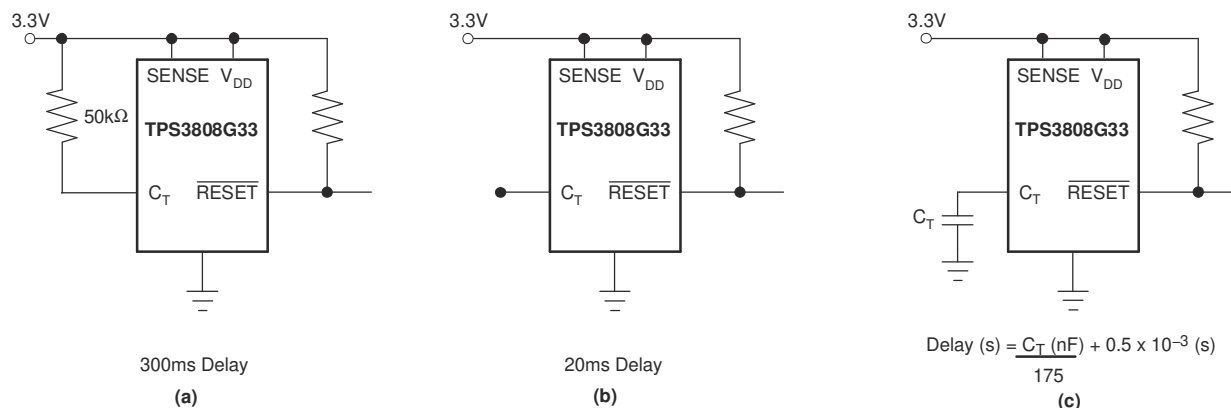
Figure 7-2. Configuration Used to Set the \overline{\text{RESET}} Delay Time
