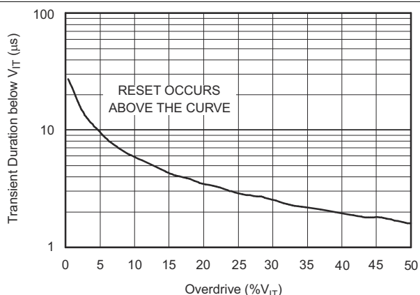
Figure 6-5. Maximum Transient Duration at Sense vs Sense Threshold Overdrive Voltage
