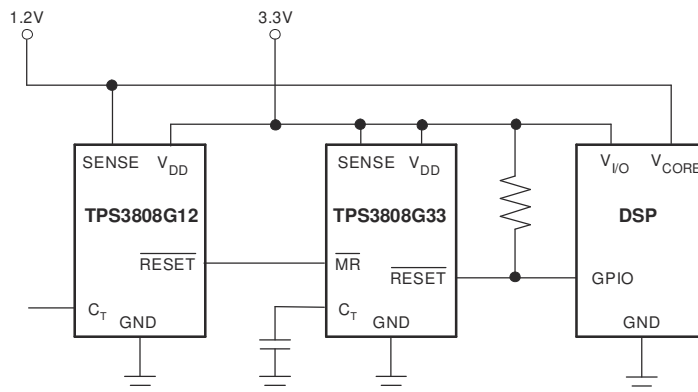
Figure 7-3. Using \overline{\text{MR}} to Monitor Multiple System Voltages
