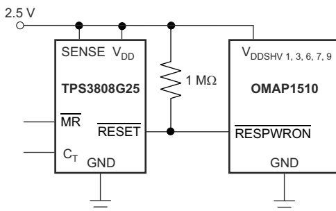
Figure 8-1. Typical Application of the TPS3808 With an OMAP™ Processor
