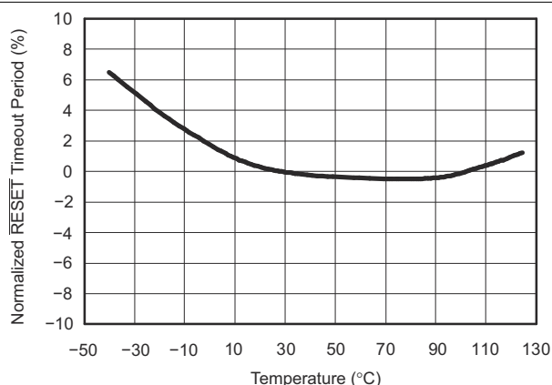
Figure 6-4. Normalized RESET Time-Out Period vs Temperature ( C_T = \text{Open} , C_T = V_{DD} , C_T = \text{Any} )
