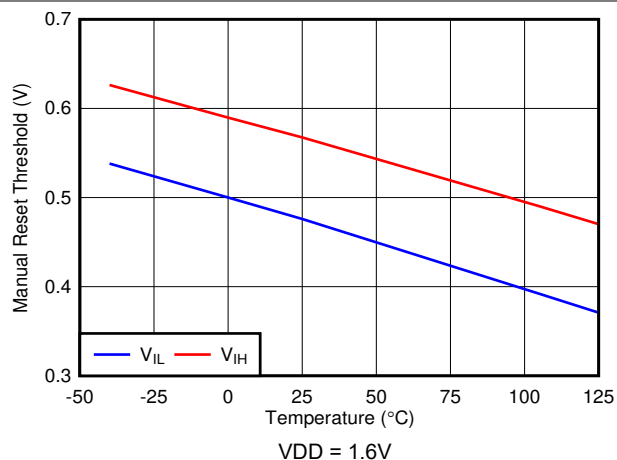
Figure 5-4. \overline{MR} Threshold vs Temperature
