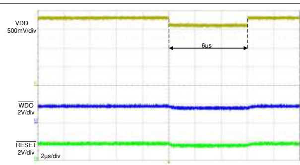
Figure 7-8. High-to-Low Glitch Immunity
