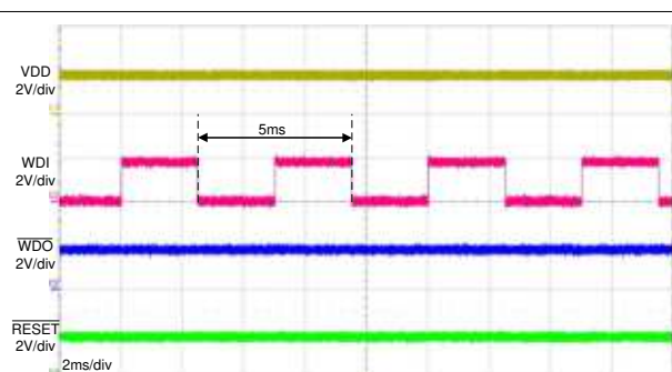
Figure 7-6. Typical WDI Signal
