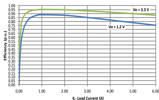
Efficiency vs Load Current, Vin = 5 V
