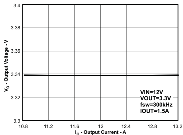
Figure 62. Regulation Versus Input Voltage
