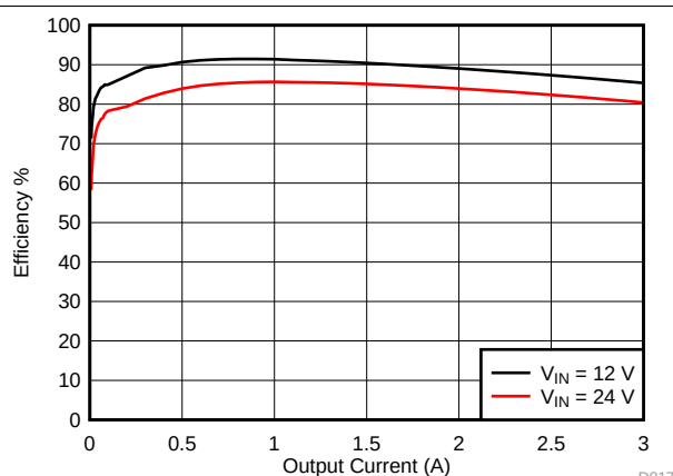
Figure 20. TPS54334 Efficiency
