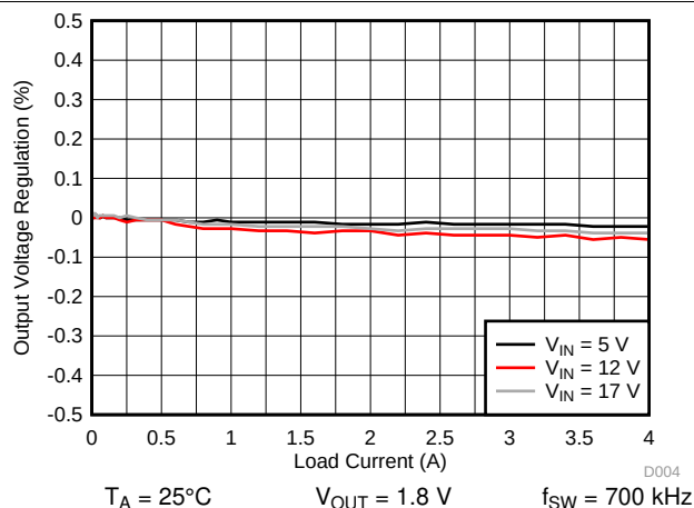
Figure 38. Load Regulation
