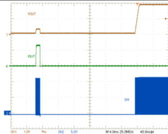
Figure 51. Output Short Circuit Response
