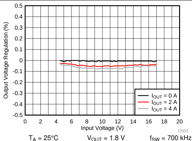
Figure 39. Line Regulation
