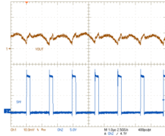
Figure 43. Output Ripple, Full Load
