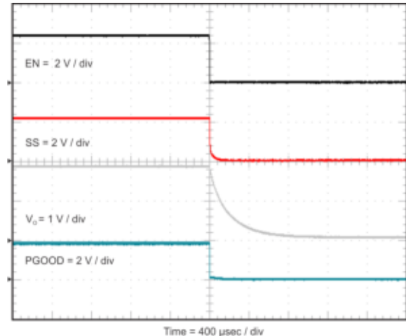
Figure 49. EN Shutdown
