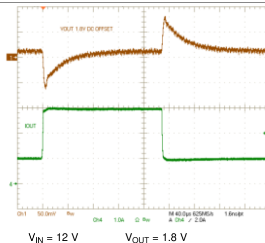
Figure 41. Transient Response
