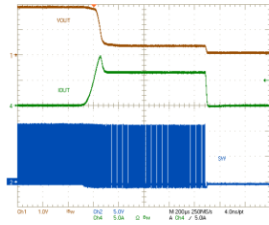
Figure 49. EN Shutdown
