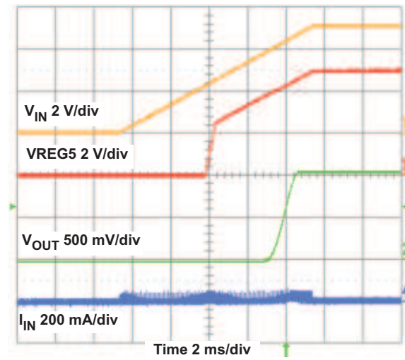
Figure 18. TPS54427 Start-Up Relative to V_{IN}
