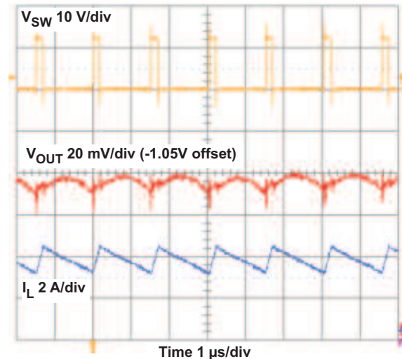
Figure 16. TPS54427 Output Voltage Ripple
