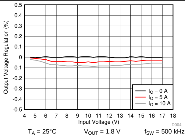
Figure 41. Line Regulation
