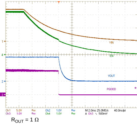
Figure 49. V_{IN} Shutdown
