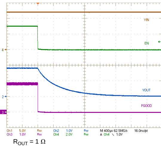
Figure 51. EN Shutdown
