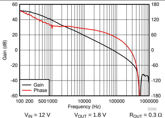
Figure 42. Loop Response
