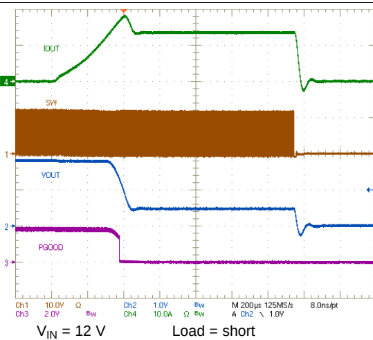
Figure 53. Output Short-Circuit Response
