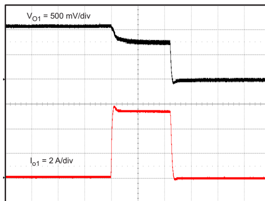
Figure 18. Overcurrent Protection, Buck 1
