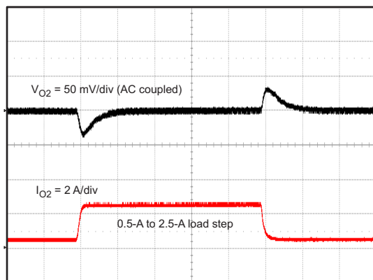
Figure 17. Load Transient, Buck 2 (0.5 A to 2.5 A)
