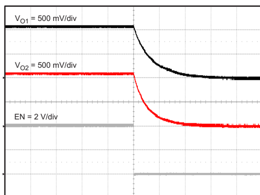
Figure 15. Shutdown With Enable
