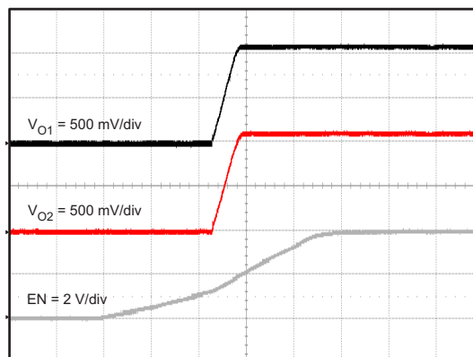
Figure 14. Startup With Enable
