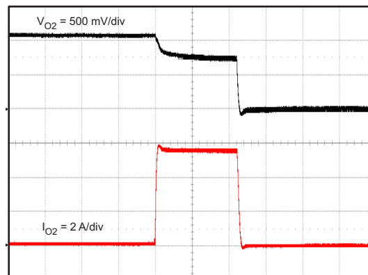
Time = 500 μs/div Figure 20. Overcurrent Protection, Buck 2
