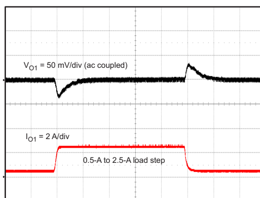
Figure 16. Load Transient, Buck 1 (0.5 A to 2.5 A)
