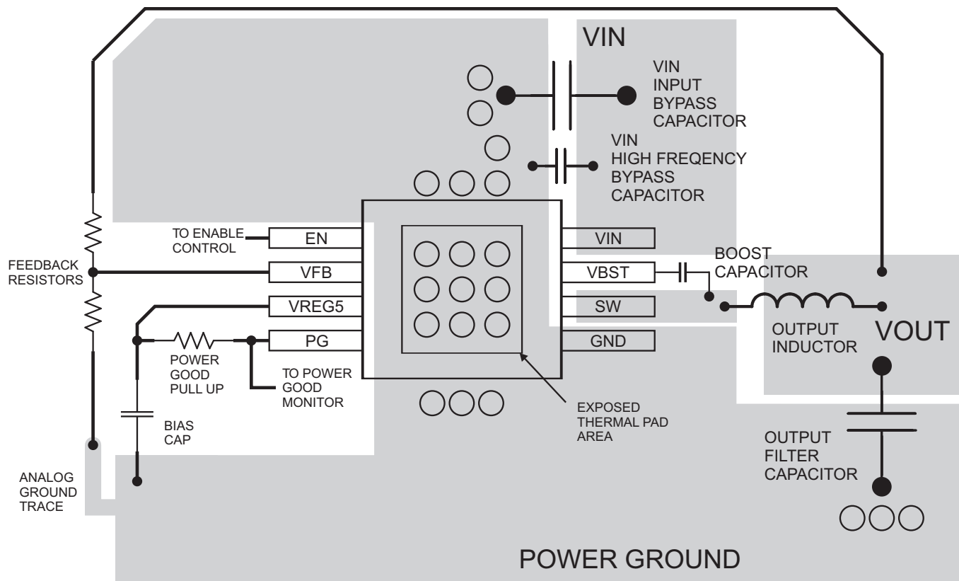
○ VIA to Ground Plane Figure 17. TPS56428 Layout – HSOP (DDA) Package
