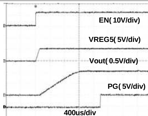
Figure 10. Slow Start
