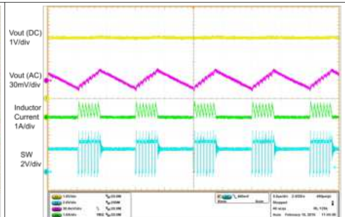
Figure 13. Switching Waveform at Light Load
