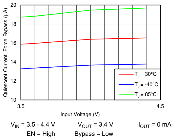
Figure 8-7. Quiescent Current at Forced Bypass Mode vs Input Voltage
