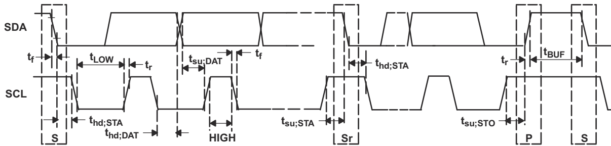
Figure 8-1. Serial Interface Timing Diagram for Standard-, Fast-, Fast-Mode Plus
