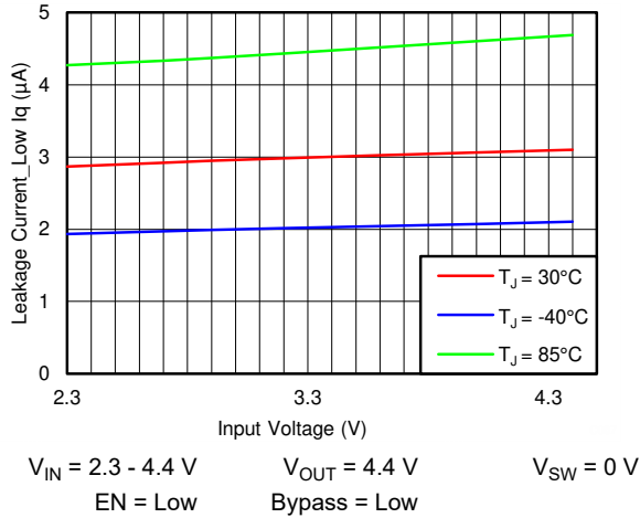
Figure 8-9. Shutdown Current at Low I Q mode vs Input Voltage
