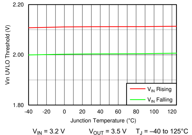
Figure 8-12. V IN UVLO Threshold Rising/Falling vs Junction Temperature
