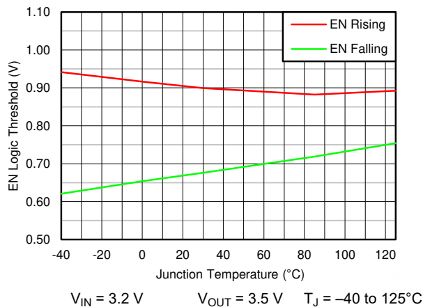
Figure 8-13. EN Logic High Threshold Rising/Falling vs Junction Temperature
