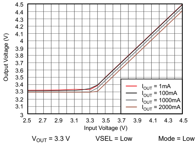
Figure 10-30. TPS61282D DC Output Voltage vs Input Voltage
