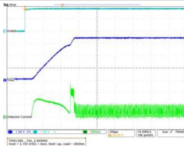
Figure 10-20. Start-Up at 30-Ω Load
