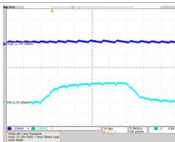
Figure 10-35. TPS61282D Line Transient
