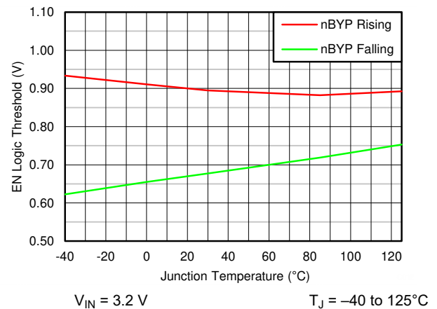
Figure 8-14. B̅YP Logic High Threshold Rising/Falling vs Junction Temperature
