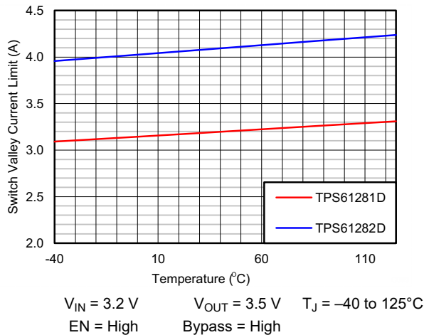
Figure 8-11. Switch Valley Current Limit: TPS61281D, TPS61282D vs Input Voltage
