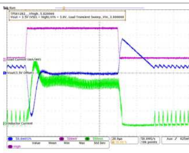
Figure 10-37. TPS61282D Load Transient Response In PFM/PWM Operation
