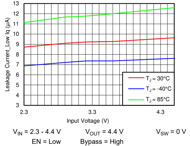
Figure 8-10. Shutdown Current vs Input Voltage
