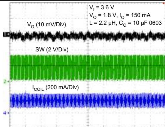
Figure 19. Typical Operation (PWM Mode)
