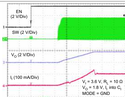
Figure 23. Start-Up Timing
