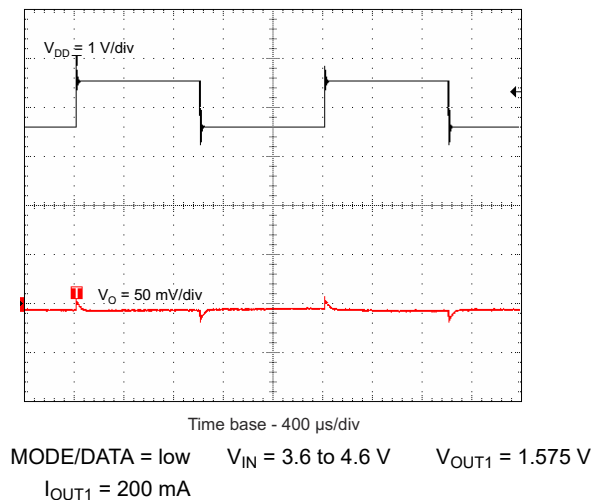
Figure 9-19. Line-Transient Response
