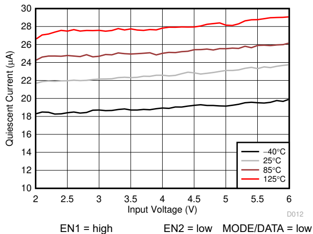
Figure 7-2. TPS62407-Q1 Quiescent Current, One Converter On
