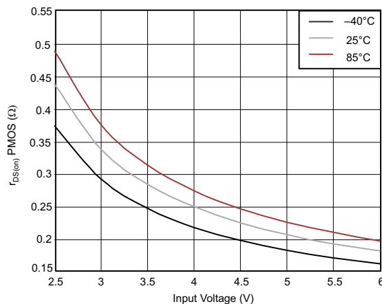
Figure 7-4. r_{\text{DS(on) PMOS}} vs V_{\text{IN}}
