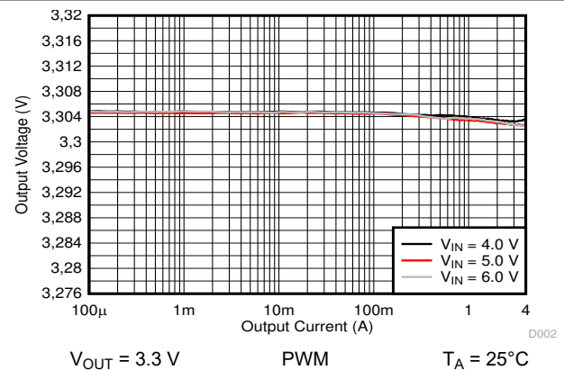
Figure 9-13. Output Voltage versus Output Current
