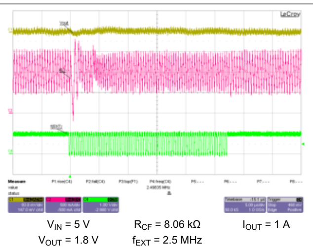
Figure 9-62. Switching from External Synchronization to Internal Fixed Frequency
