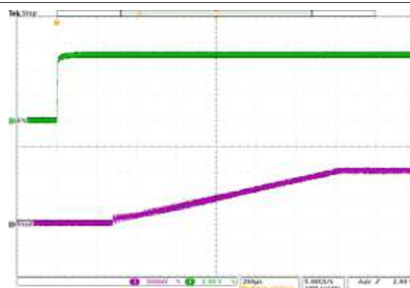
Figure 9-53. Start-Up Timing
