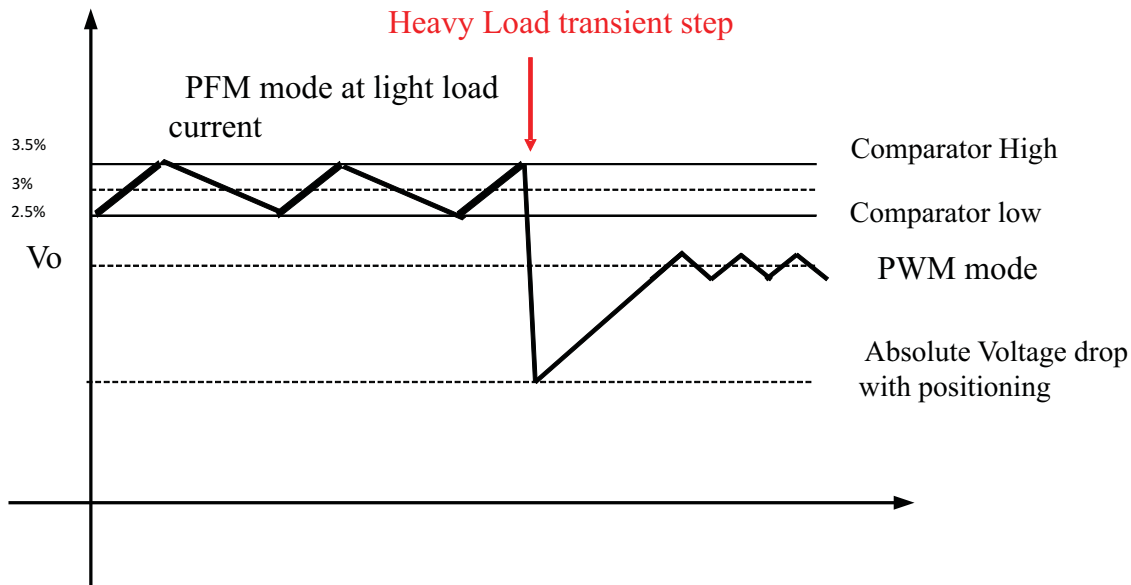
Figure 19. Power-Save Mode Thresholds and Dynamic Voltage Positioning
