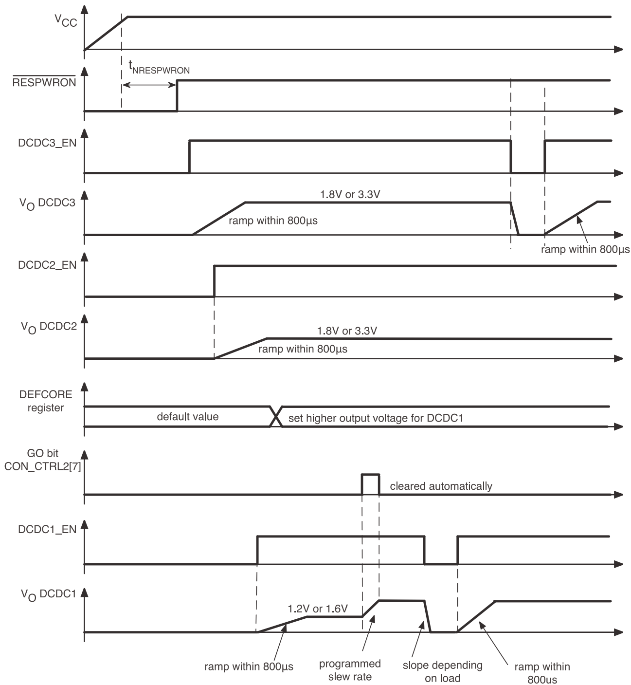
Figure 4. DVS Timing
