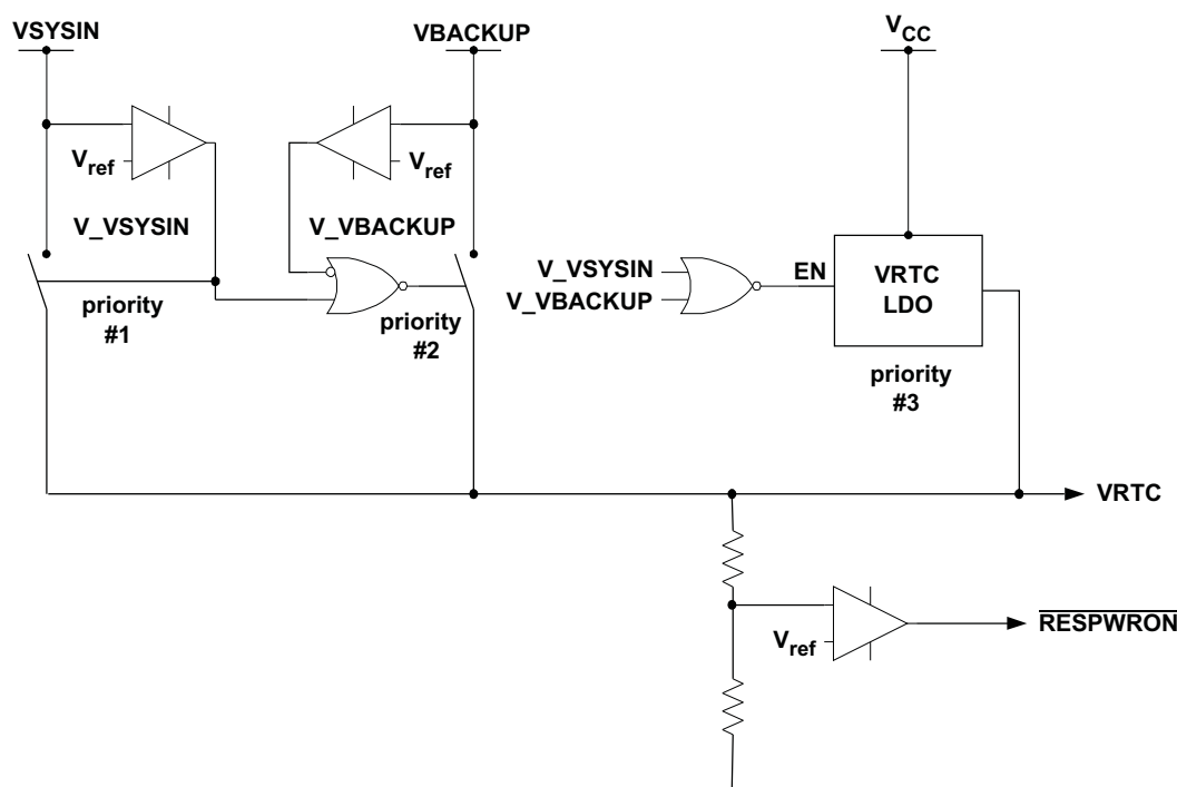
Figure 32. RTC and RESPWRON
