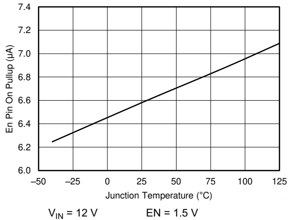
Figure 6-13. EN Pin Pullup Current vs Temperature, EN = 1.5\text{ V}
