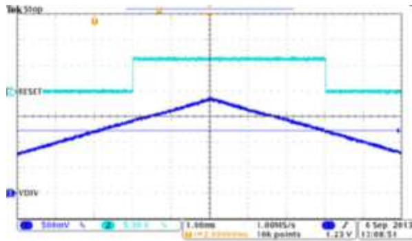
Figure 8-33. Trigger Voltage 1.23V, Reset vs VDIV
