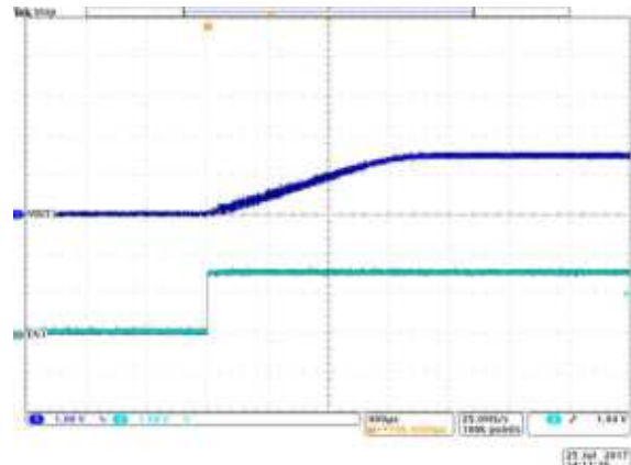
Figure 8-3. BUCK1 Soft-Start
