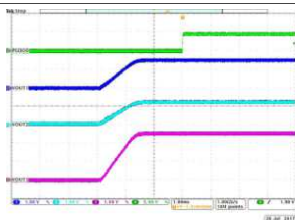
Figure 8-18. PGOOD
