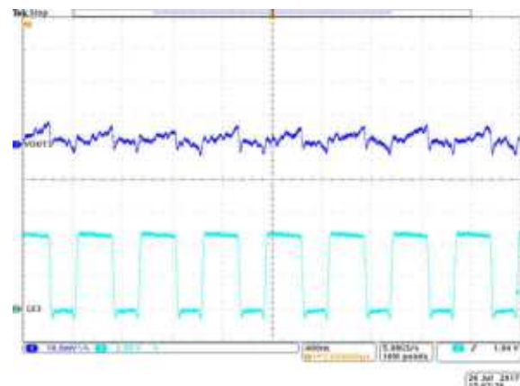
Figure 8-6. BUCK1 Output Voltage Ripple
