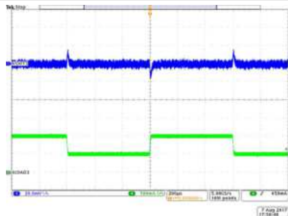
Figure 8-11. BUCK2 Load Transient
