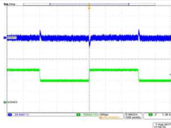
Figure 8-12. BUCK2 Load Transient
