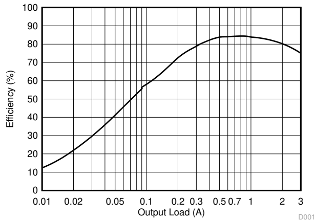
Figure 6-1. BUCK1 Efficiency
