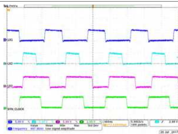
Figure 8-20. Synchronization With External Clock
