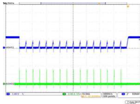
Figure 8-16. BUCK2 Hiccup and Recovery
