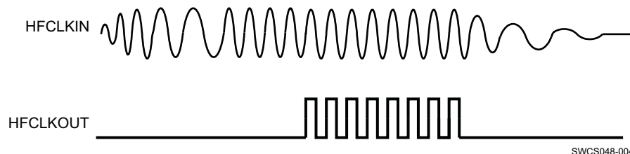
Figure 4-4. HFCLKOUT Behavior
