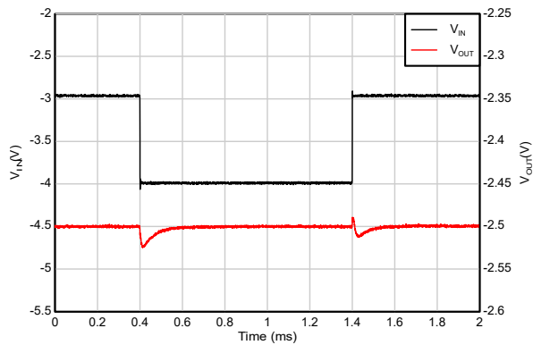
Figure 5-37. TPS72325 Line Transient Response (new chip)
