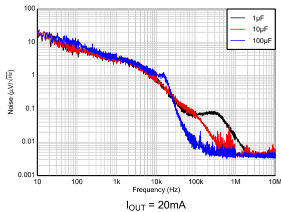
Figure 5-65. TPS72325 Total Noise vs C_{OUT} (10Hz to 10MHz) (New chip)
