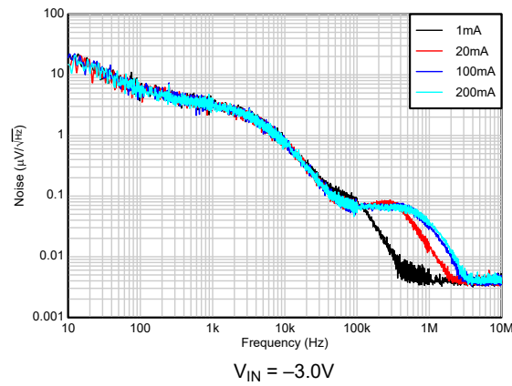
Figure 5-61. TPS72325 Total Noise vs I_{OUT} (10Hz to 10MHz) (New chip)
