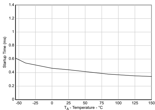
Figure 5-50. TPS72325 Start-up time vs Temp (new chip)
