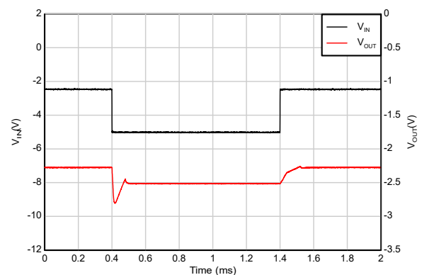
Figure 5-39. TPS72325 Line Transient Response (new chip)
