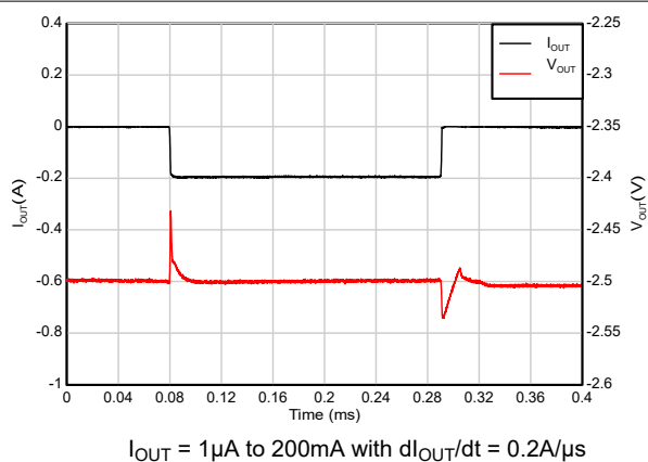
Figure 5-45. TPS72325 Load Transient Response (new chip)
