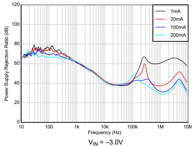
Figure 7-9. PSRR vs I_{OUT} (New chip)
