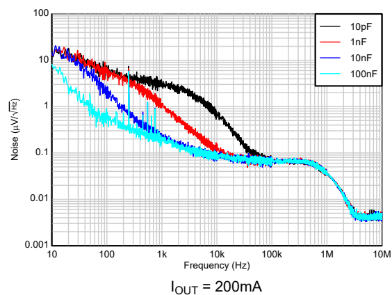
Figure 5-59. TPS72325 Total Noise vs C_{NR} (10Hz to 10MHz) (New chip)
