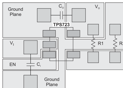
Figure 7-10. Example Layout
