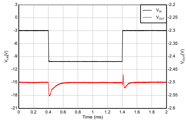
Figure 5-38. TPS72325 Line Transient Response (new chip)
