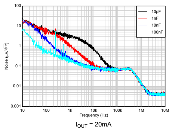
Figure 5-60. TPS72325 Total Noise vs C_{NR} (10Hz to 10MHz) (New chip)
