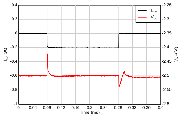
Figure 5-44. TPS72325 Load Transient Response (new chip)
