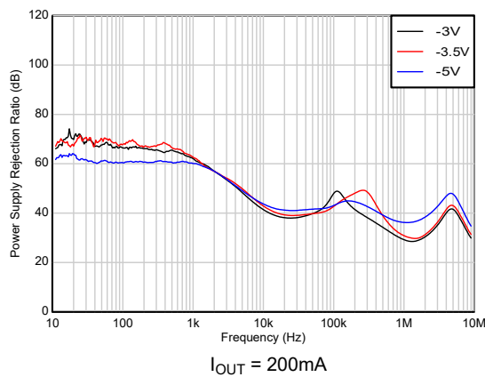
Figure 5-75. PSRR vs V_{IN} (New chip)
