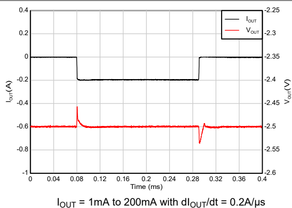
Figure 5-46. TPS72325 Load Transient Response (new chip)
