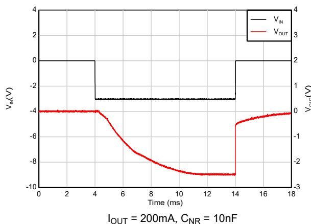
Figure 7-7. TPS72325 Start-up Response ( V_{IN} & EN tied together) (New chip)
