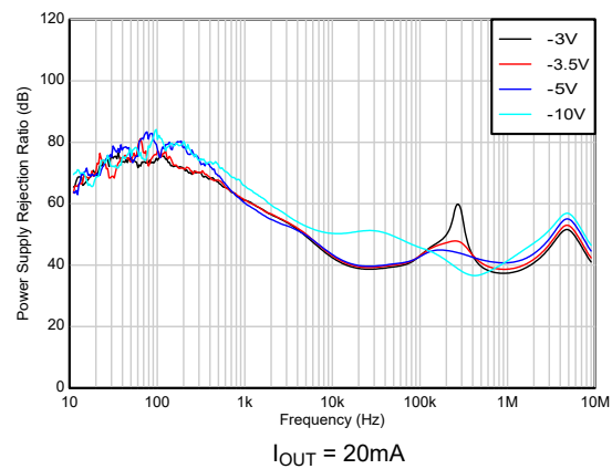
Figure 5-76. PSRR vs V_{IN} (New chip)
