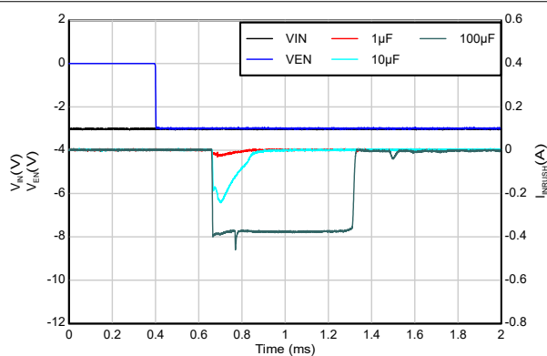
Figure 5-55. TPS72325 Start-up Response ( V_{IN} & EN tied together) (New chip)
