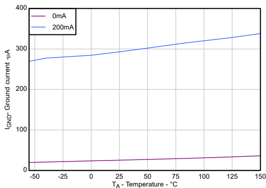
Figure 5-17. Ground Current vs Junction Temperature (new chip)
