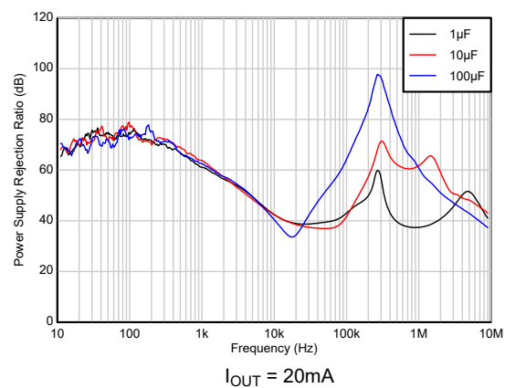
Figure 5-78. PSRR vs C_{OUT} (New chip)
