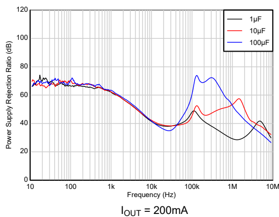
Figure 5-77. PSRR vs C_{OUT} (New chip)
