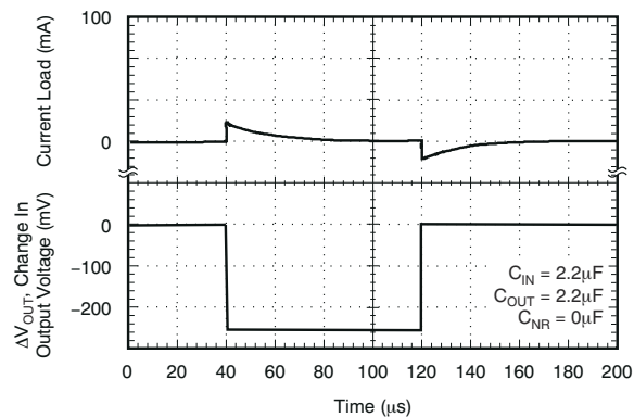
Figure 5-43. TPS72325 Load Transient Response (legacy chip)
