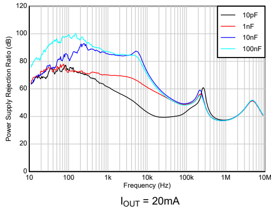
Figure 5-73. PSRR vs C_{NR} (New chip)
