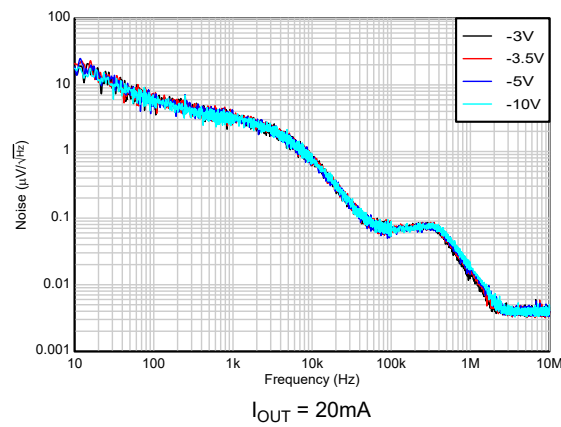
Figure 5-63. TPS72325 Total Noise vs V_{IN} (10Hz to 10MHz) (New chip)
