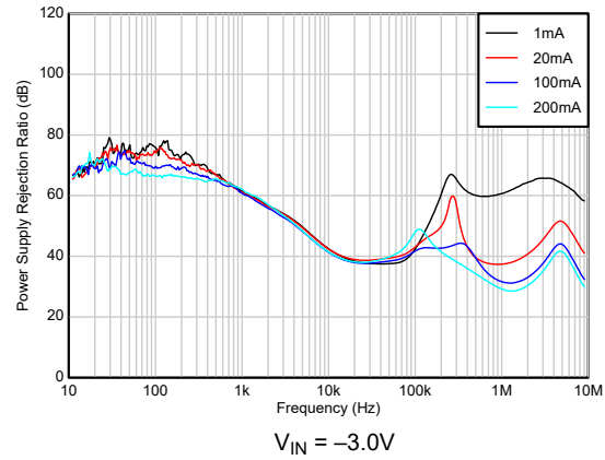
Figure 5-74. PSRR vs I_{OUT} (New chip)
