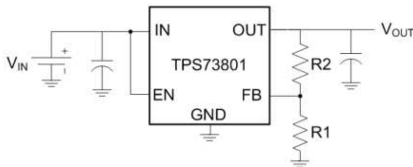
Simplified Application
