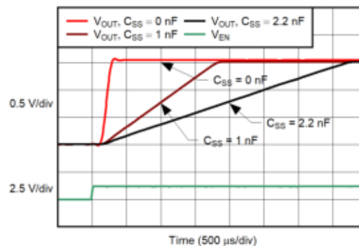
Figure 5-38. Turn-On Response
