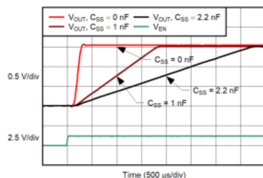
Turn-On Response
