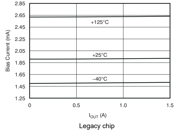
Figure 5-22. I_{BIAS} vs I_{OUT} and Temperature
