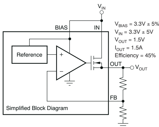
Figure 7-2. Typical Application of the TPS742 Without an Auxiliary Bias
