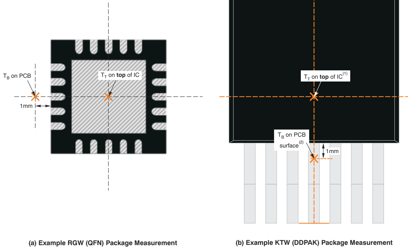
Figure 7-9. Measuring Points for T_T and T_B
