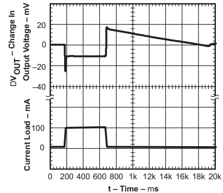
Figure 26. TPS79118 Load Transit Response
