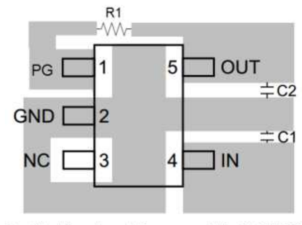
Figure 16. Layout Example
