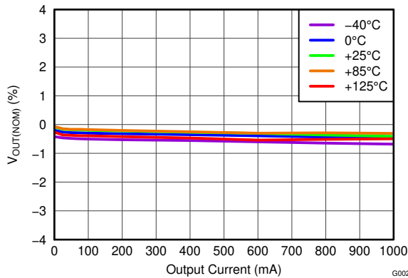
Figure 5-3. Load Regulation
