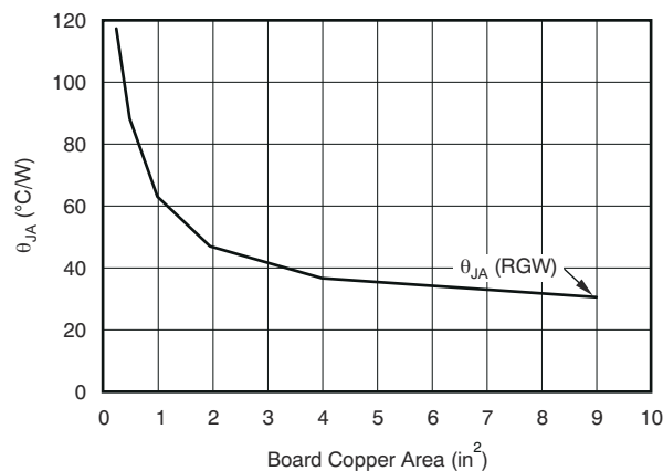
Figure 8-1. \theta_{JA} vs Board Size
