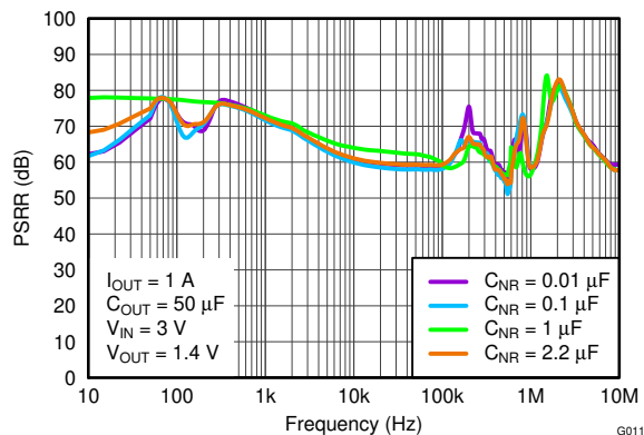
Figure 5-11. Power-Supply Rejection Ratio vs C_{\text{NR}}
