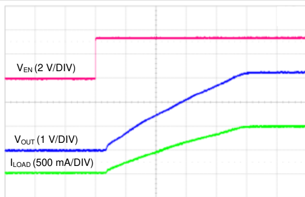
Figure 7-2. Startup with EN Pin rising (10 ms/DIV)
