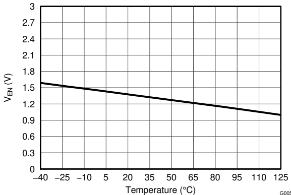
Figure 5-5. Enable Voltage Threshold vs Temperature
