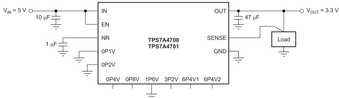
Figure 7-1. Typical Application, V_{OUT} = 3.3\text{ V}
