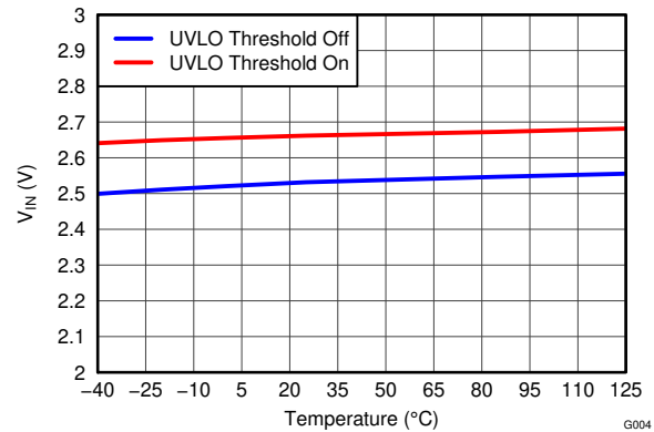
Figure 5-4. UVLO Threshold vs Temperature
