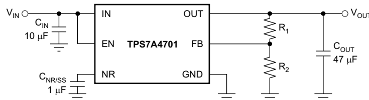
Figure 6-1. Adjustable Operation for Maximum AC Performance
