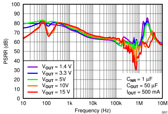
Figure 5-17. Power-Supply Rejection Ratio vs Output Voltage
