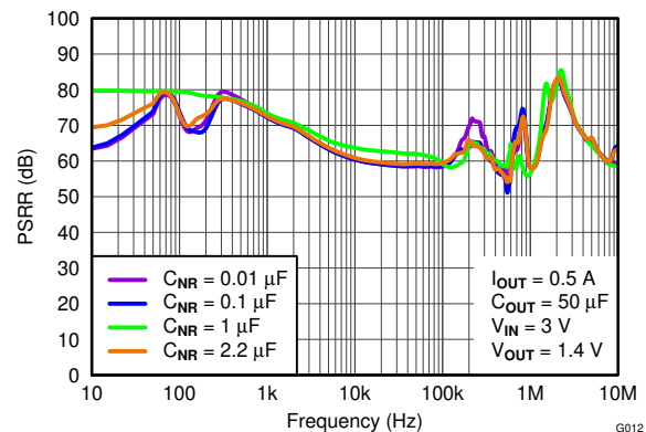
Figure 5-12. Power-Supply Rejection Ratio vs C_{\text{NR}}
