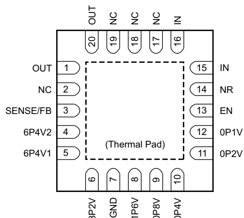
Figure 4-1. RGW Package 5-mm × 5-mm VQFN-20 (Top View)
