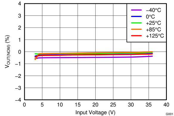
Figure 5-2. Line Regulation
