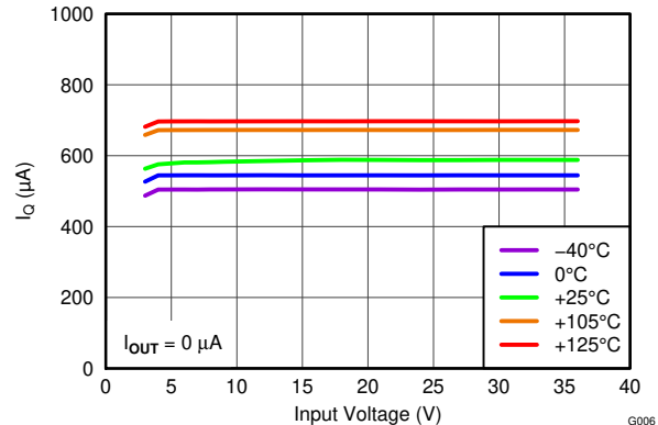
Figure 5-6. Quiescent Current vs Input Voltage
