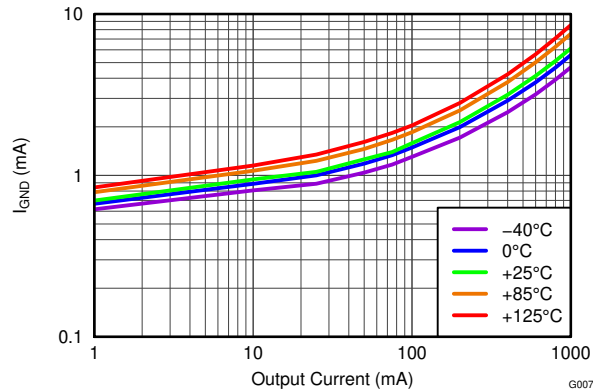
Figure 5-7. Ground Current vs Output Current
