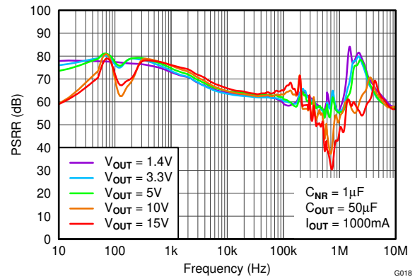
Figure 5-18. Power-Supply Rejection Ratio vs Output Voltage
