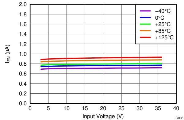
Figure 5-8. Enable Current vs Input Voltage
