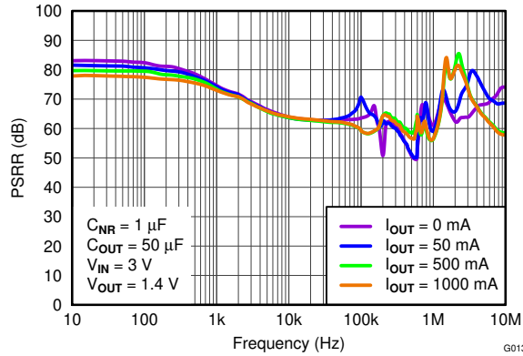
Figure 5-13. Power-Supply Rejection Ratio vs I_O
