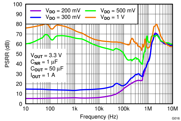
Figure 5-16. Power-Supply Rejection Ratio vs Dropout
