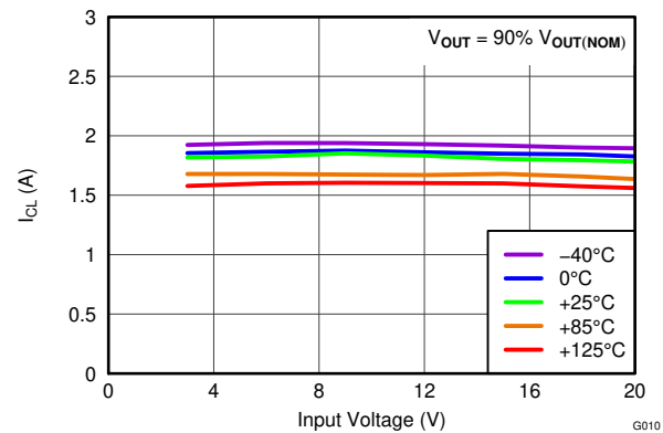
Figure 5-10. Current Limit vs Input Voltage
