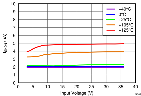
Figure 5-9. Shutdown Current vs Input Voltage
