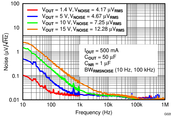
Figure 5-1. Noise vs Output Voltage
