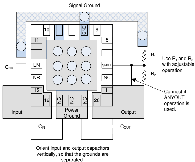
Figure 9-1. Layout Example
