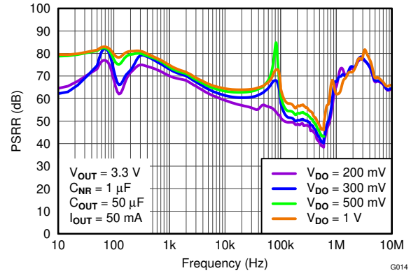
Figure 5-14. Power-Supply Rejection Ratio vs Dropout
