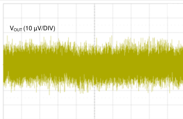
Figure 7-3. Output Noise Voltage, 10 Hz to 100 kHz (10 ms/DIV)
