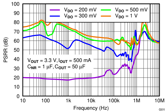
Figure 5-15. Power-Supply Rejection Ratio vs Dropout
